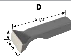
1.5 lbs. Part #15058 (681)
