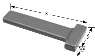
1.82 lbs. Part #15031 (678)
