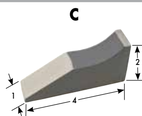
1.25 lbs. Part #15012 (647)
