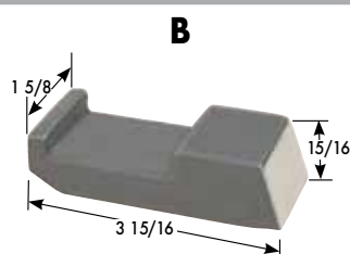
1.25 lbs. Part #15001 (638)
