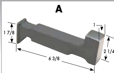
2 lbs. Part #15000 (670)
