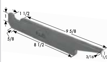
2 lbs. Part #15004 (649)
