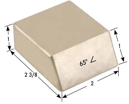
2.87 lbs. Part #74102
