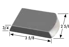
1.6 lbs. Part #15038 (724)
