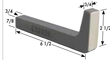
1.3 lbs. Part #15024 (612)
