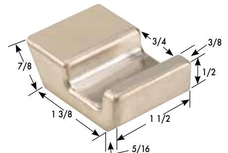
1.2 lbs. Part #74104
