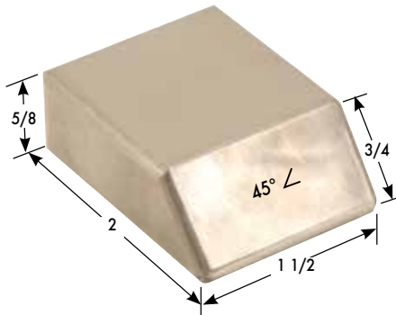
1.07 lbs. Part #74101
